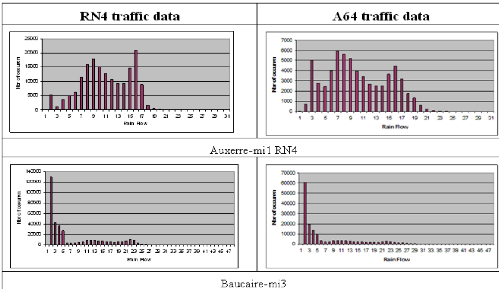
Rain-flow histograms
